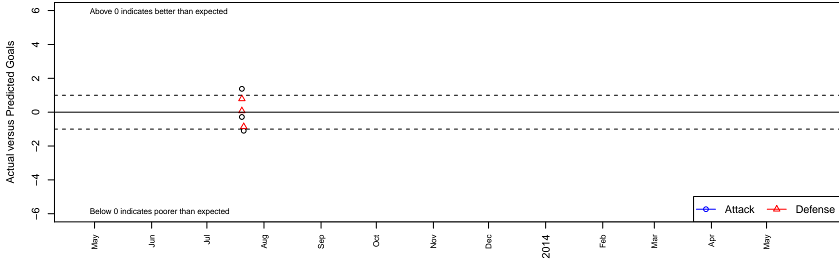
MFC Matrix -Unk G99 Dots are actual minus expected GF (blue circles) and GA (red triangles). Blue line is smoothed change in attack strength. Red is smoothed change in defense strength.
